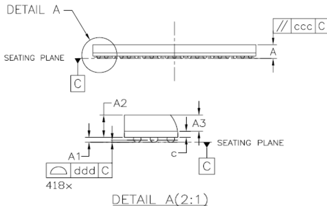
Fig.2-5 Package side view
