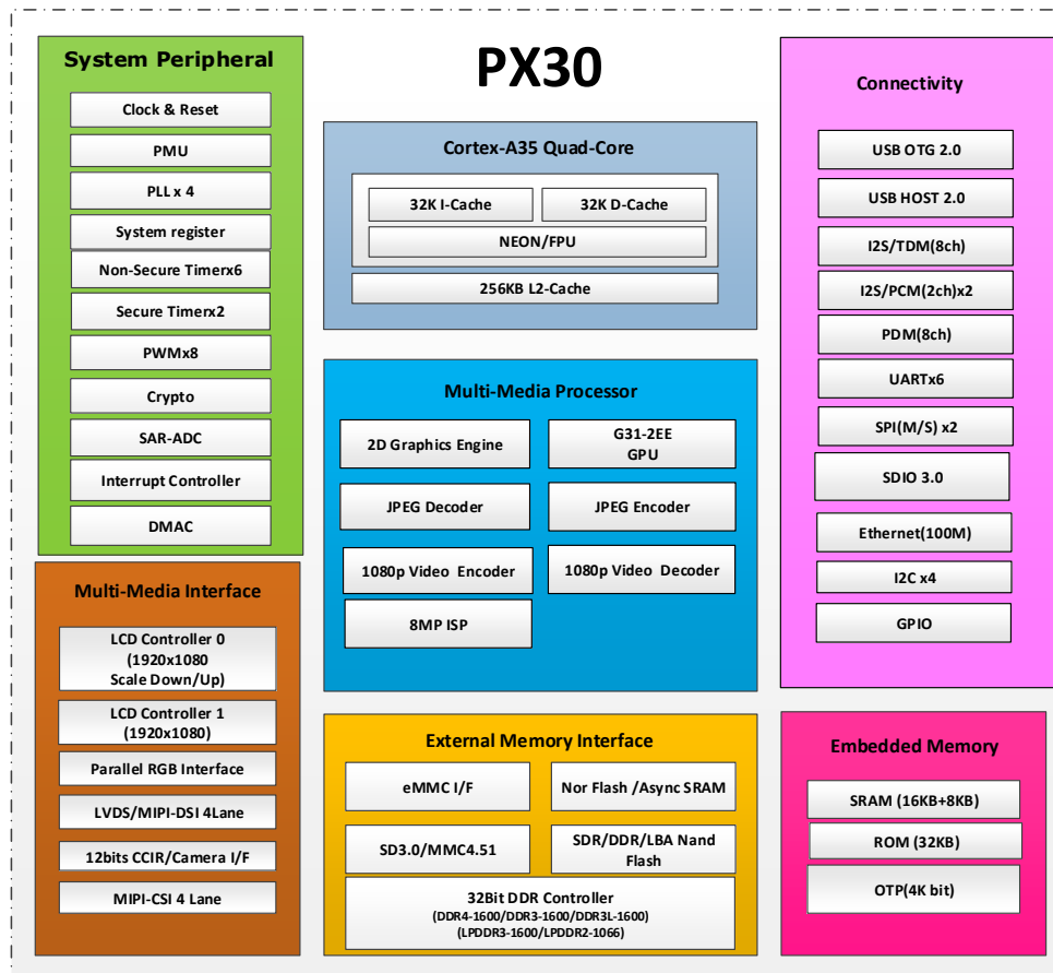
Fig.1-1 Block Diagram
